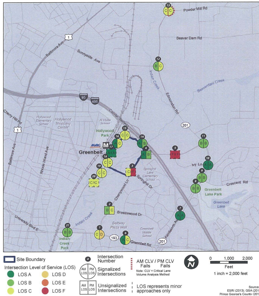
Figure ES-12: Greenbelt Build with Mitigation Condition Intersection LOS for AM and PM Peak Hours
