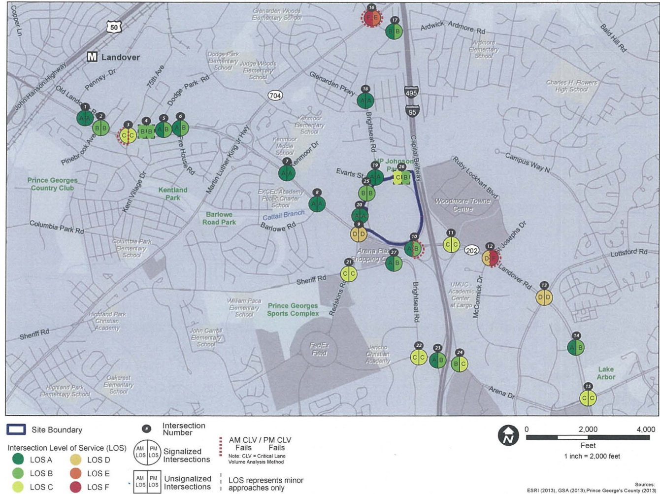
Figure ES- 14: Landover Build with Mitigation Condition Intersection LOS for AM and PM Peak Hours
